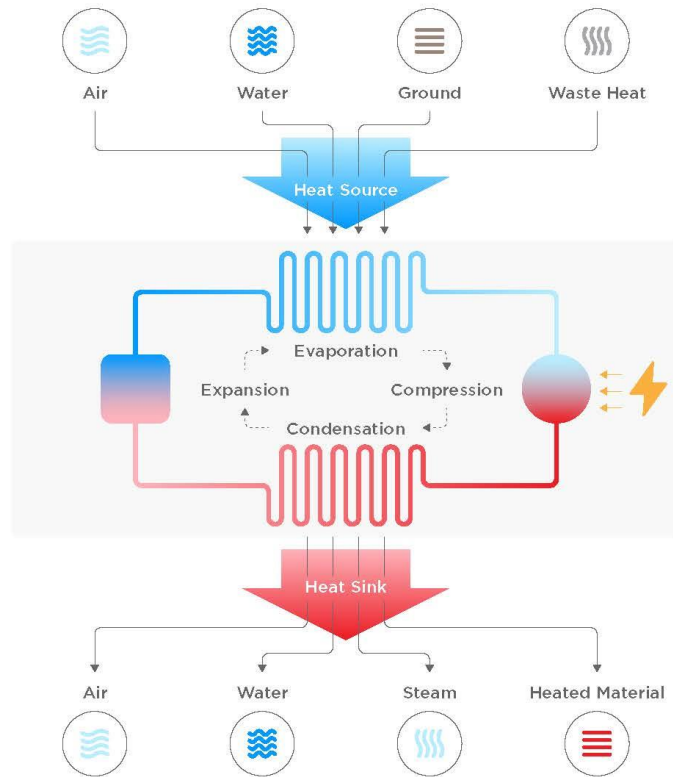
Figure 5: How Heat Pumps Work 10
