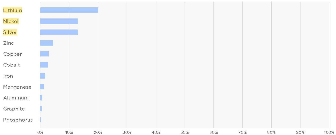
Figure 17: Materials Required Relative to 2023 USGS Estimated Resources
