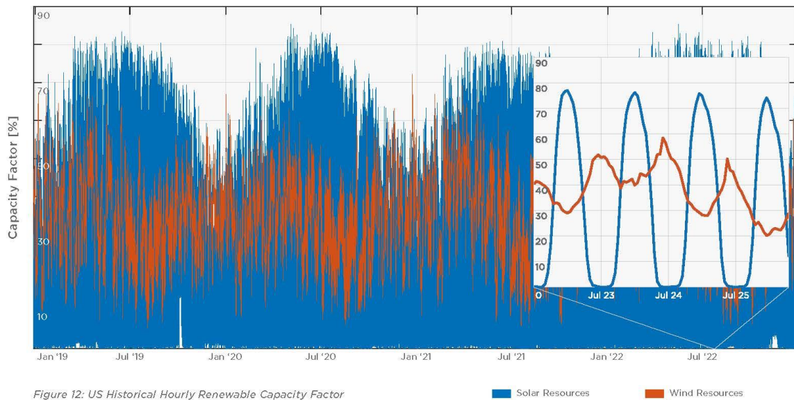
Figure 12: US Historical Hourly Renewable Capacity Factor
