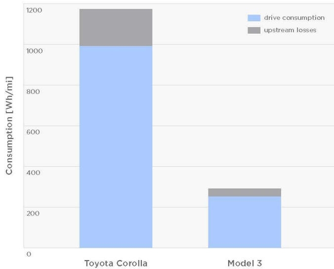
Figure 4: Comparison Tesla Model 3 vs. Toyota Corolla
