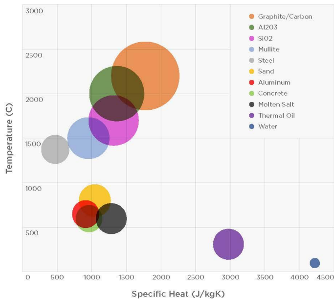
Figure 10: Thermal Storage - Heat Storage Media
